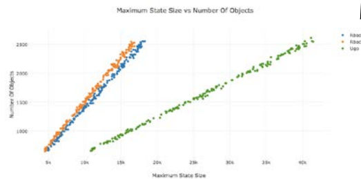
Figure 1: State size vs. Number objects
